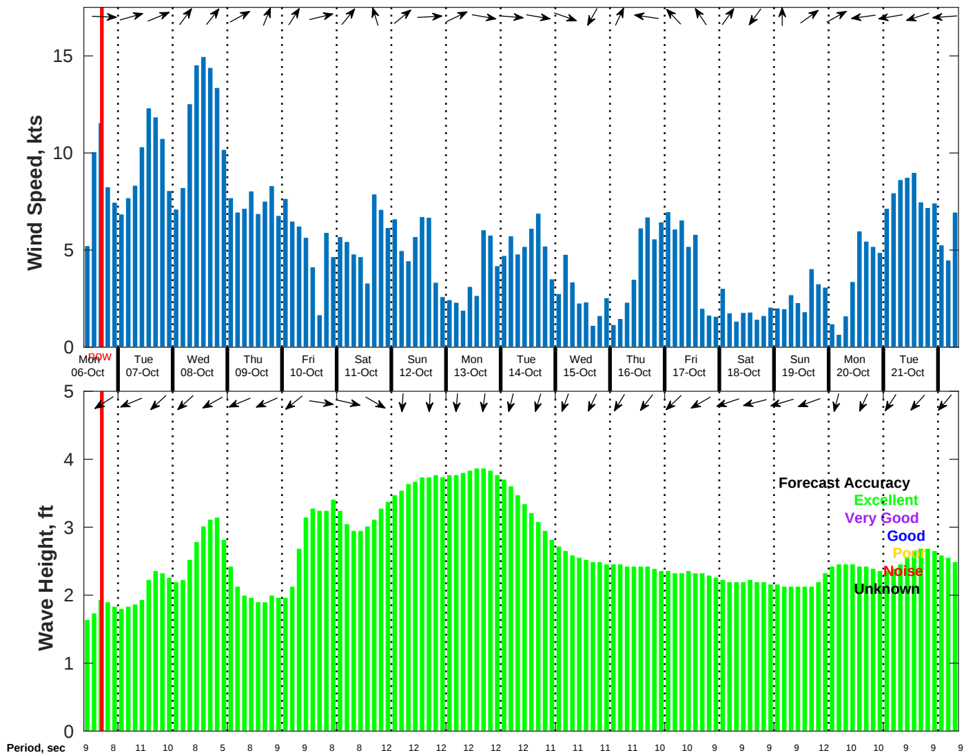
Wind & Wave Forecast for NDBC 52212 from 05-Oct-2025 09:00:00 to 21-Oct-2025 09:00:00
