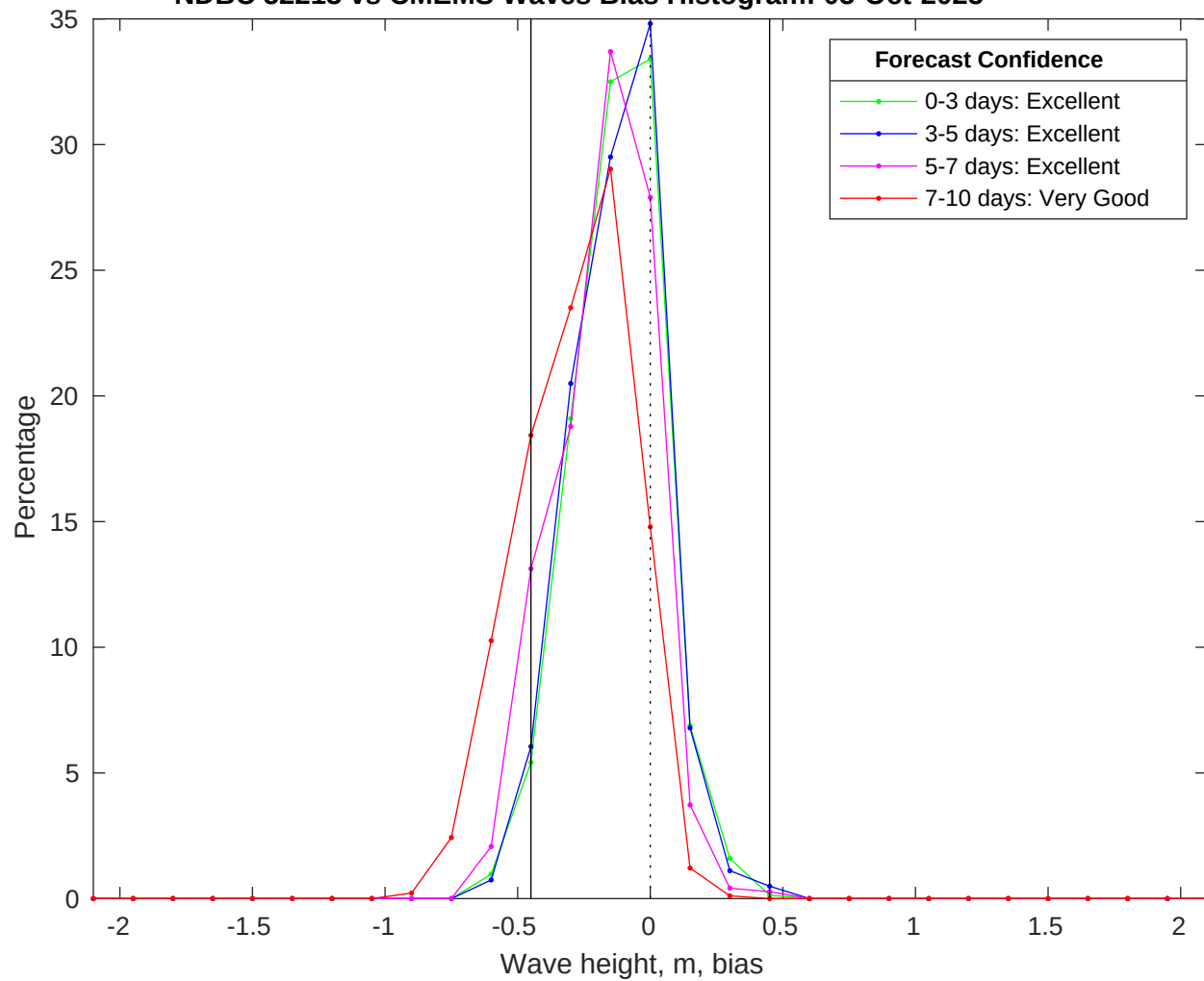
NDBC 52213 vs CMEMS Waves Bias Histogram: 05-Oct-2025
