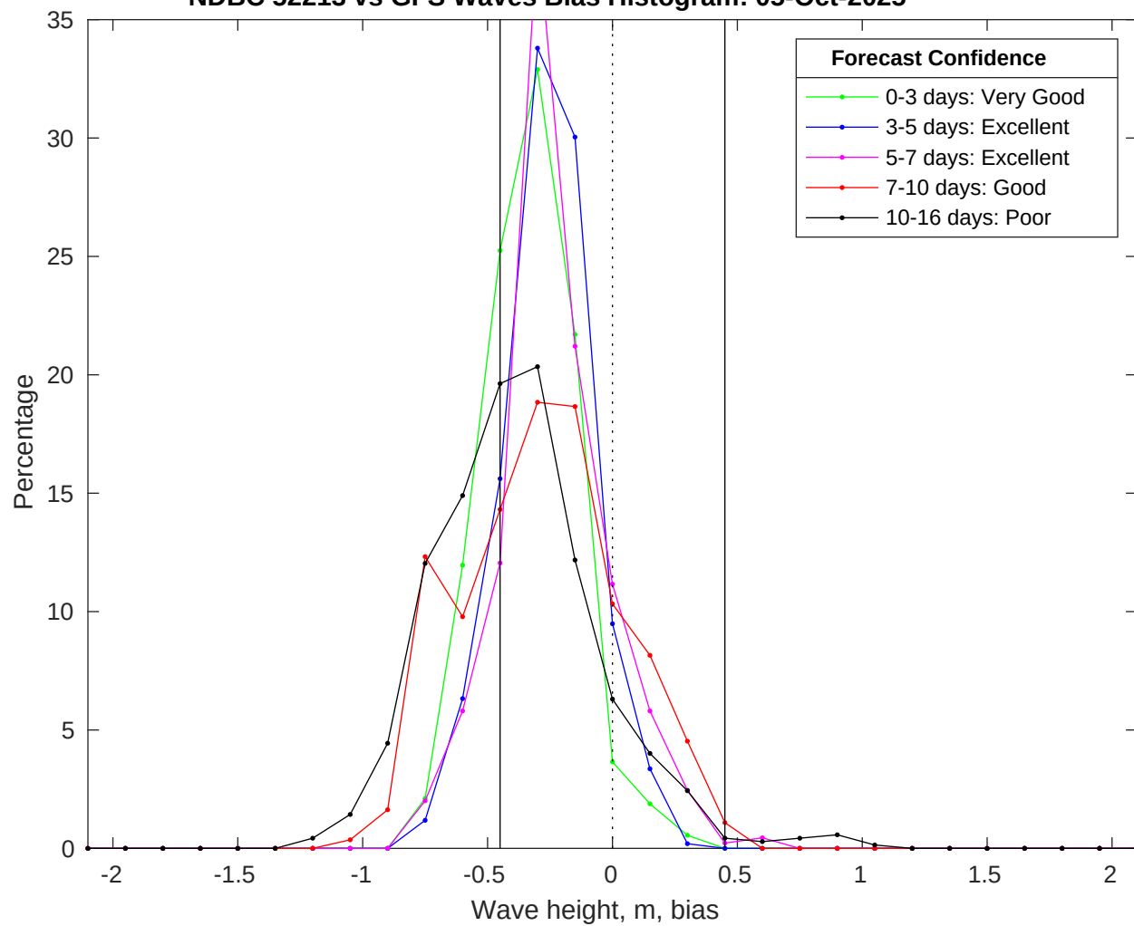
NDBC 52213 vs GFS Waves Bias Histogram: 05-Oct-2025
