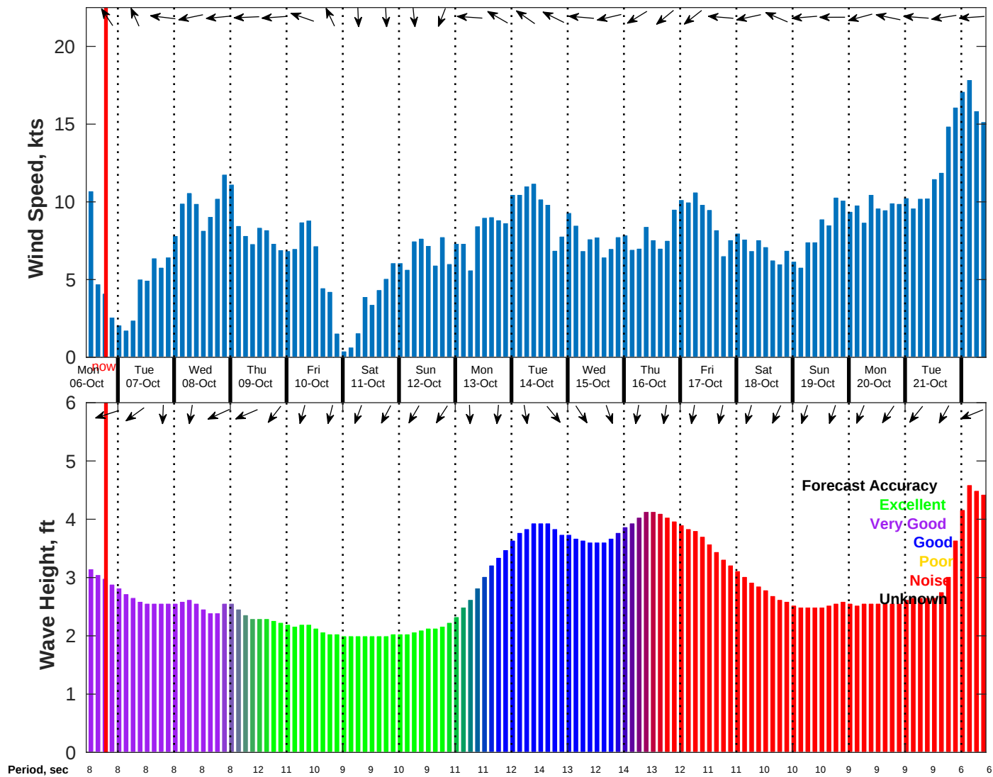
Wind & Wave Forecast for NDBC 52213 from 05-Oct-2025 11:00:00 to 21-Oct-2025 11:00:00
