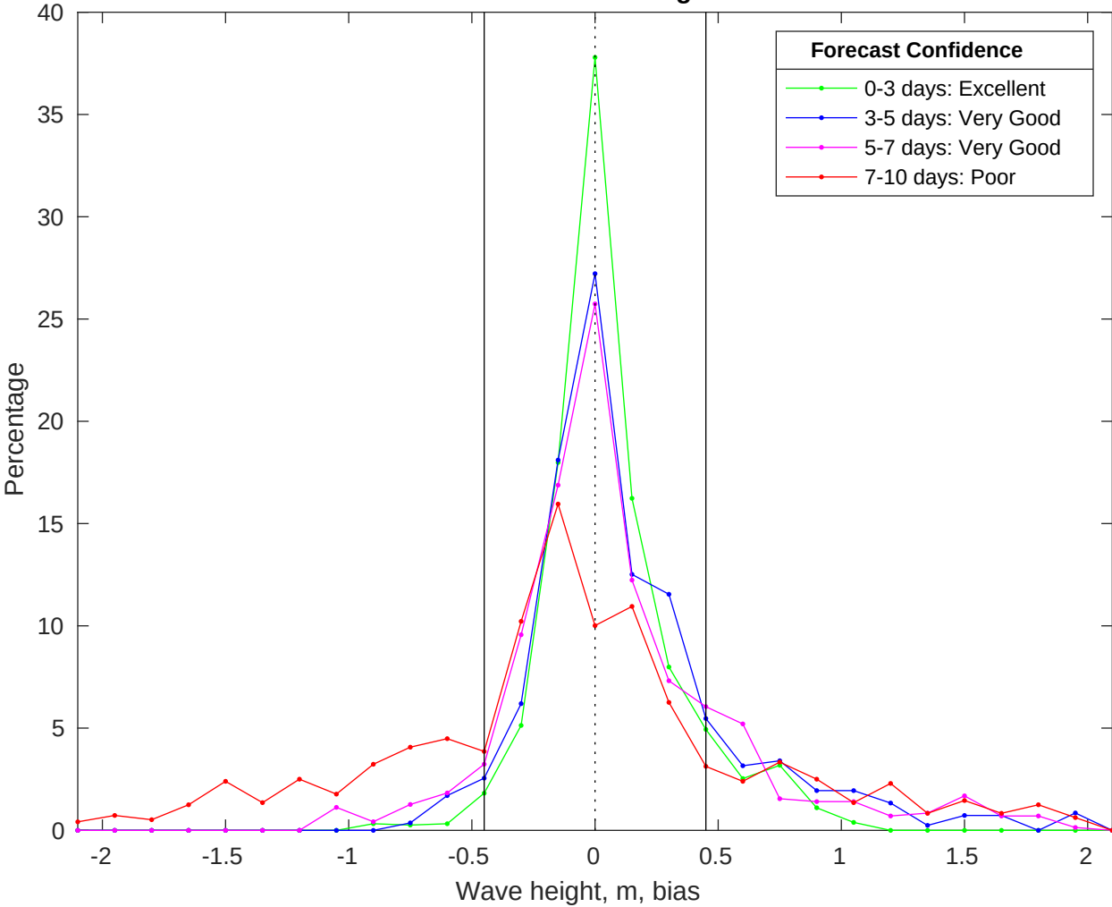
NDBC 41004 vs CMEMS Waves Bias Histogram: 06-Oct-2025
