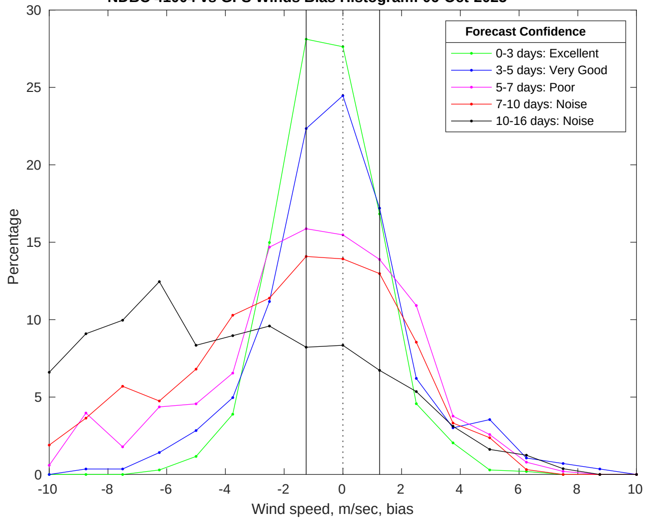
NDBC 41004 vs GFS Winds Bias Histogram: 06-Oct-2025
