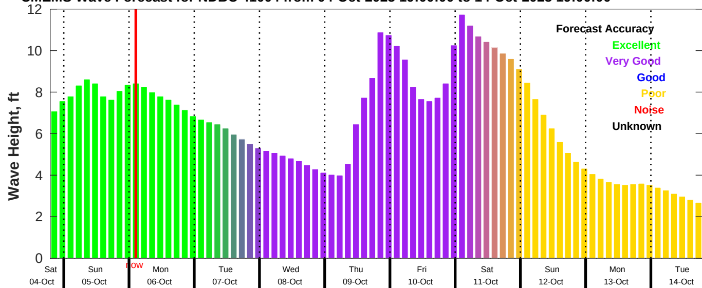
CMEMS Wave Forecast for NDBC 41004 from 04-Oct-2025 19:00:00 to 14-Oct-2025 19:00:00
