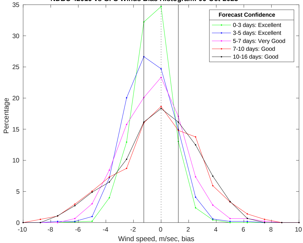
NDBC 42019 vs GFS Winds Bias Histogram: 06-Oct-2025
