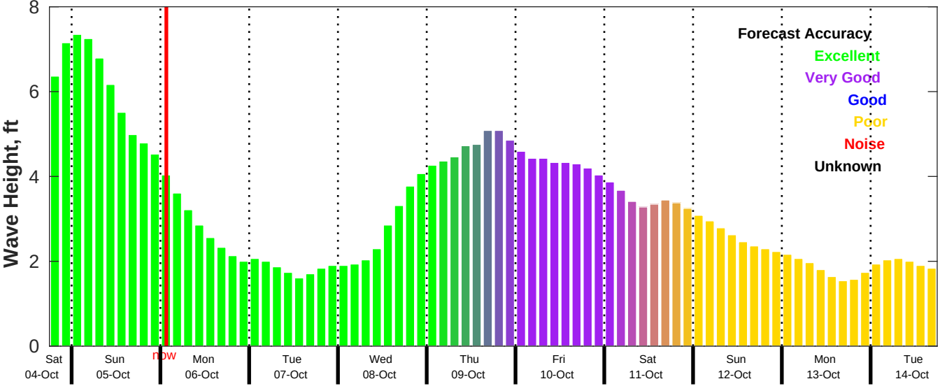
CMEMS Wave Forecast for NDBC 42019 from 04-Oct-2025 18:00:00 to 14-Oct-2025 18:00:00
