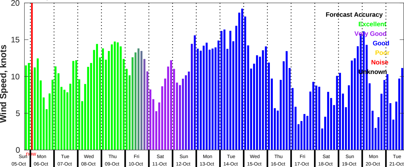
GFS Wind Speed Forecast for NDBC 42019 from 05-Oct-2025 18:00:00 to 21-Oct-2025 18:00:00
