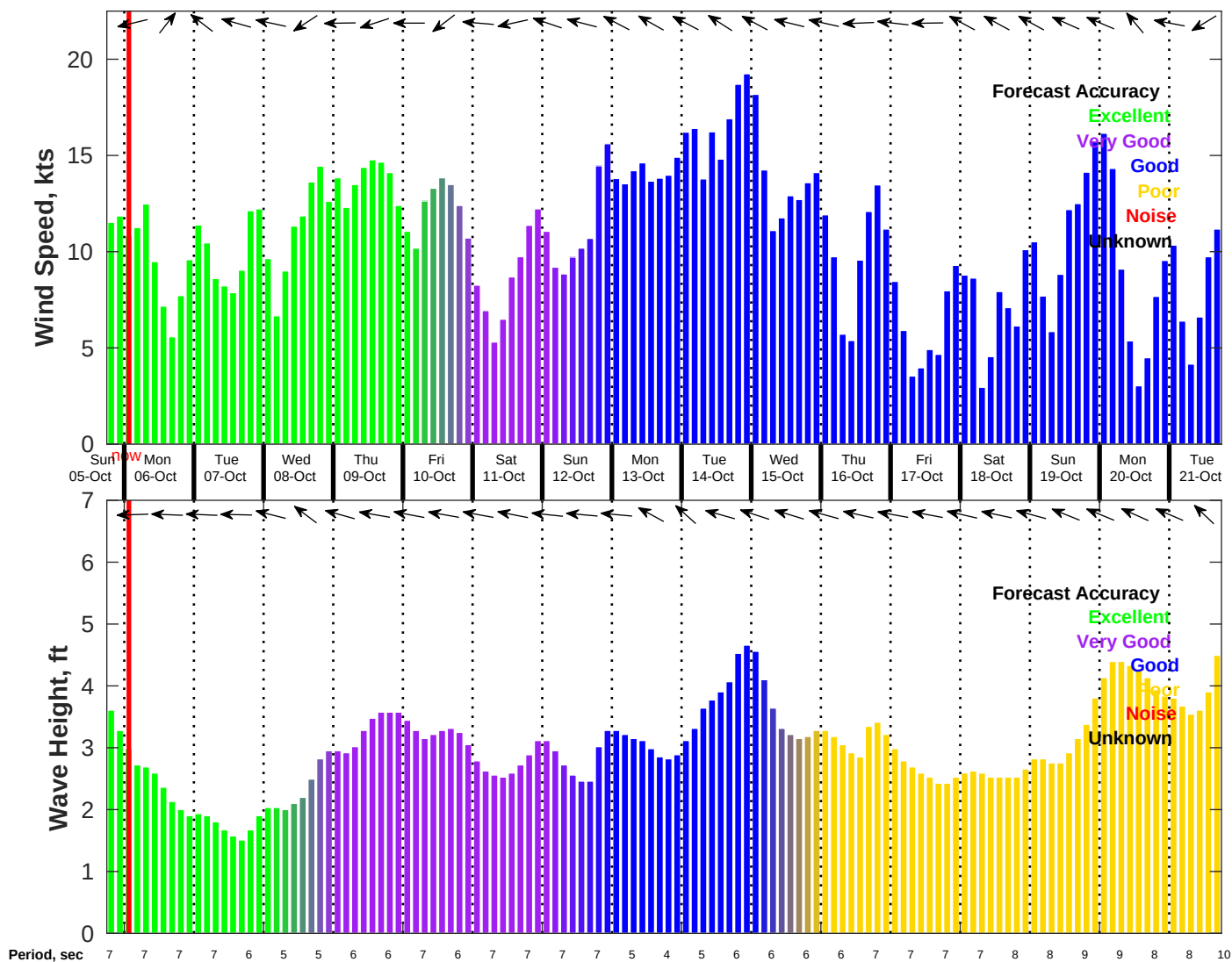
Wind & Wave Forecast for NDBC 42019 from 05-Oct-2025 18:00:00 to 21-Oct-2025 18:00:00
