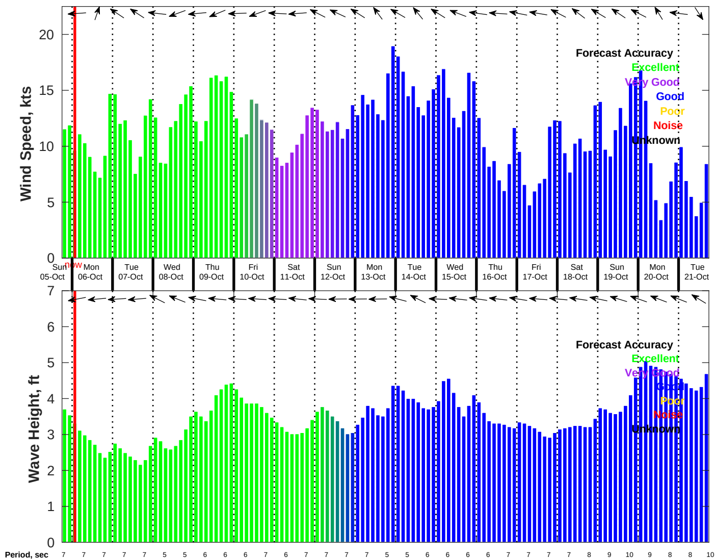
Wind & Wave Forecast for NDBC 42020 from 05-Oct-2025 18:00:00 to 21-Oct-2025 18:00:00
