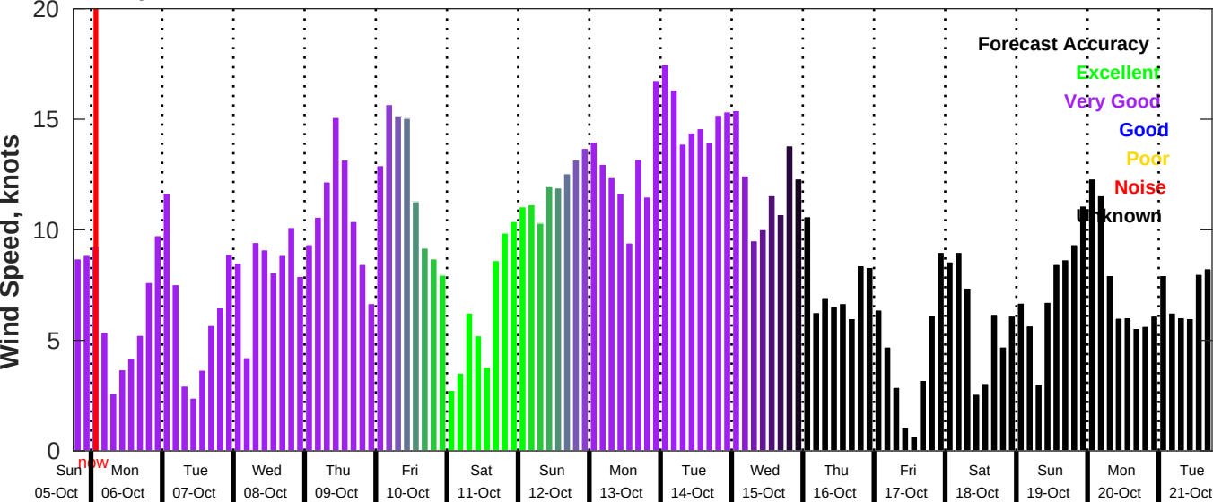
GFS Wind Speed Forecast for NDBC 42035 from 05-Oct-2025 18:00:00 to 21-Oct-2025 18:00:00
