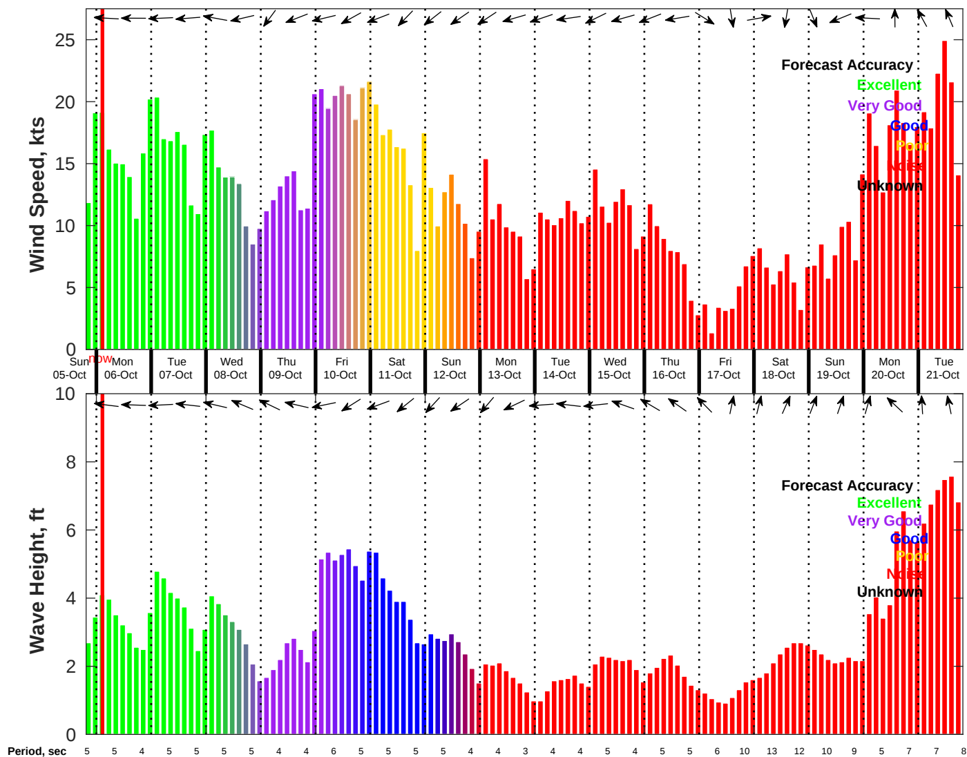
Wind & Wave Forecast for NDBC 42036 from 05-Oct-2025 19:00:00 to 21-Oct-2025 19:00:00
