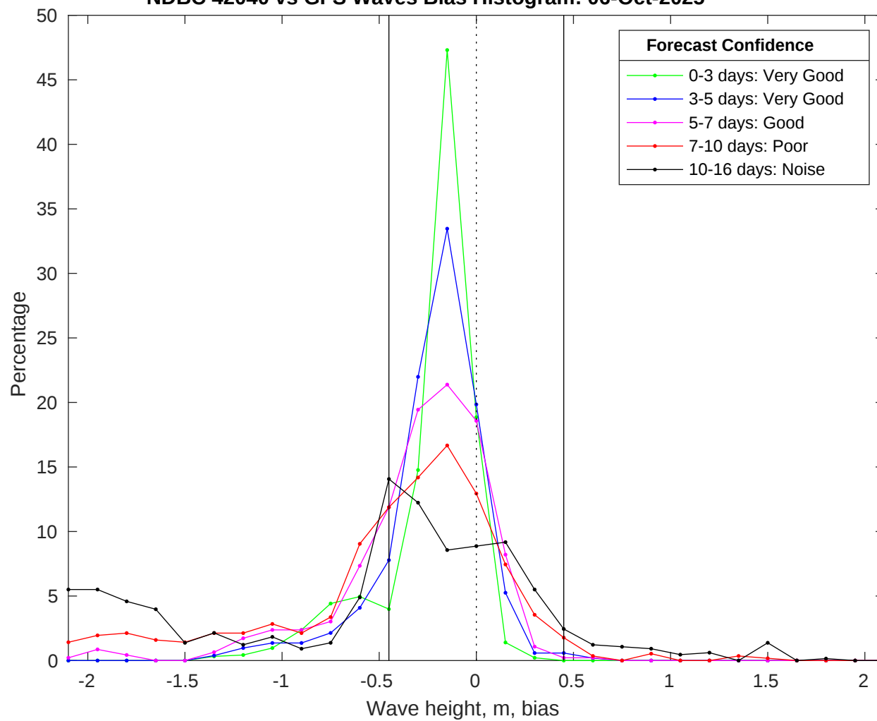
NDBC 42040 vs GFS Waves Bias Histogram: 06-Oct-2025
