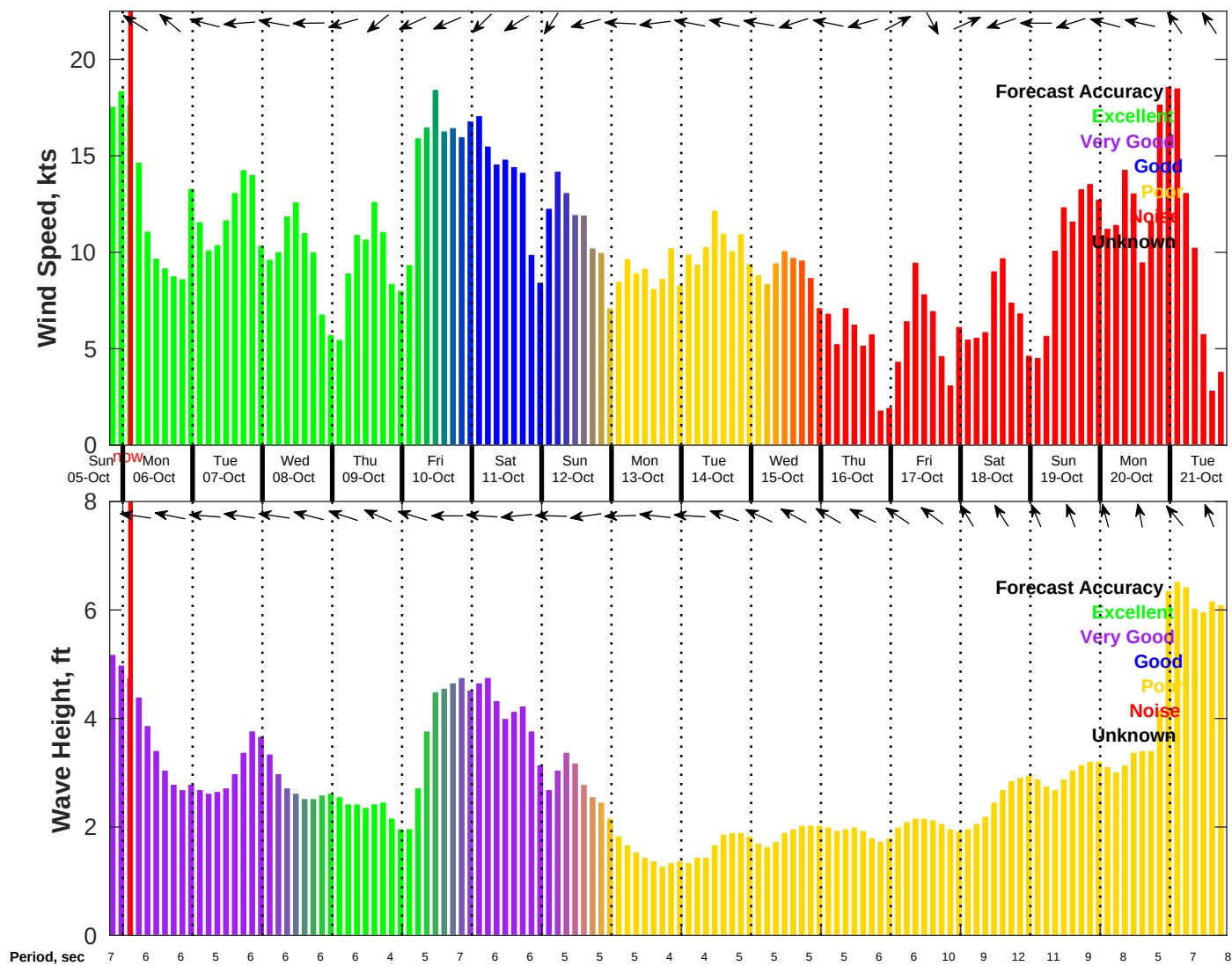
Wind & Wave Forecast for NDBC 42040 from 05-Oct-2025 19:00:00 to 21-Oct-2025 19:00:00
