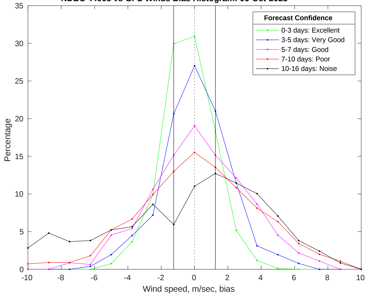
NDBC 44008 vs GFS Winds Bias Histogram: 06-Oct-2025
