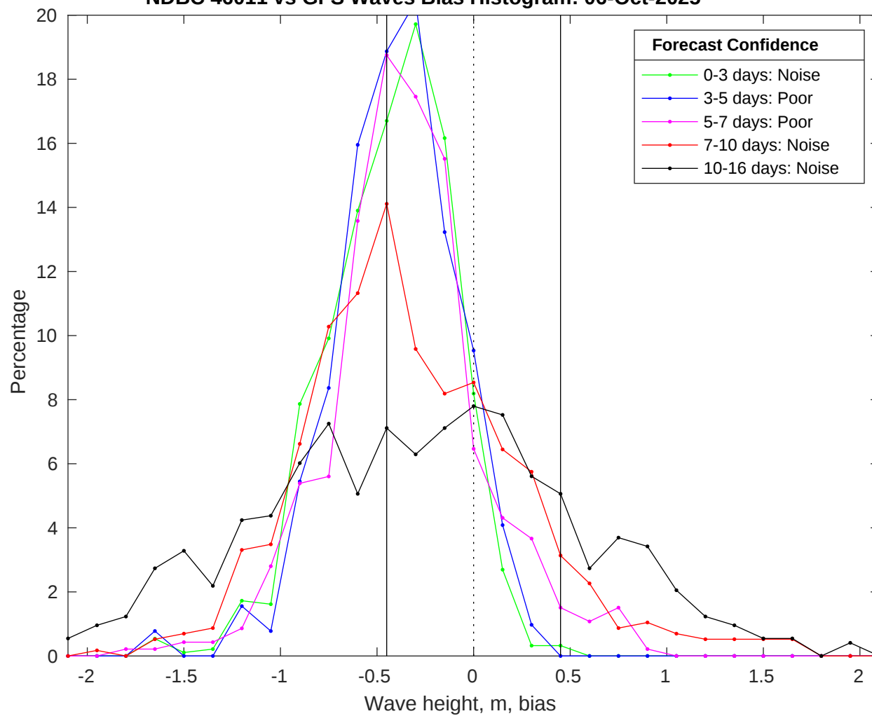
NDBC 46011 vs GFS Waves Bias Histogram: 06-Oct-2025
