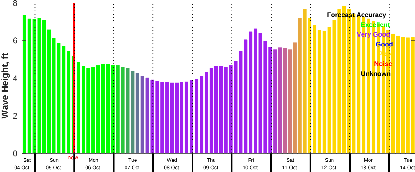
CMEMS Wave Forecast for NDBC 46011 from 04-Oct-2025 16:00:00 to 14-Oct-2025 16:00:00
