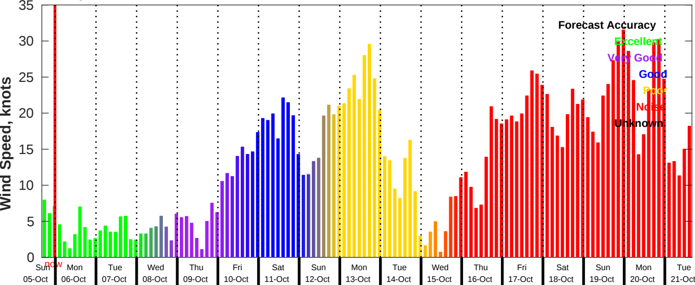
GFS Wind Speed Forecast for NDBC 46011 from 05-Oct-2025 16:00:00 to 21-Oct-2025 16:00:00
