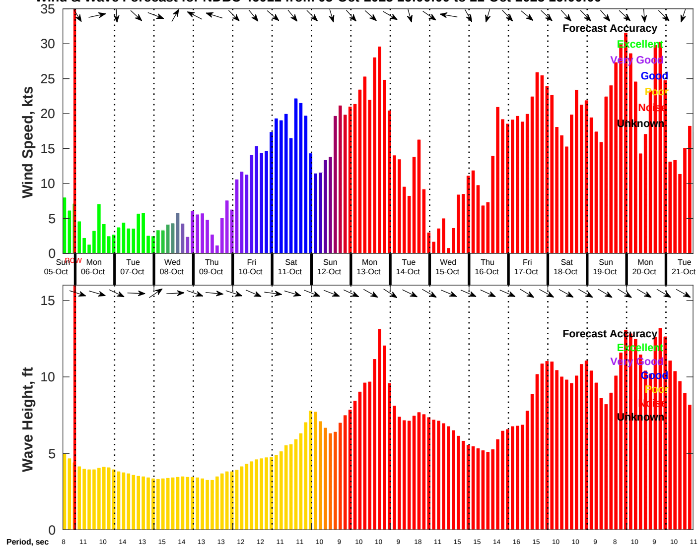
Wind & Wave Forecast for NDBC 46011 from 05-Oct-2025 16:00:00 to 21-Oct-2025 16:00:00
