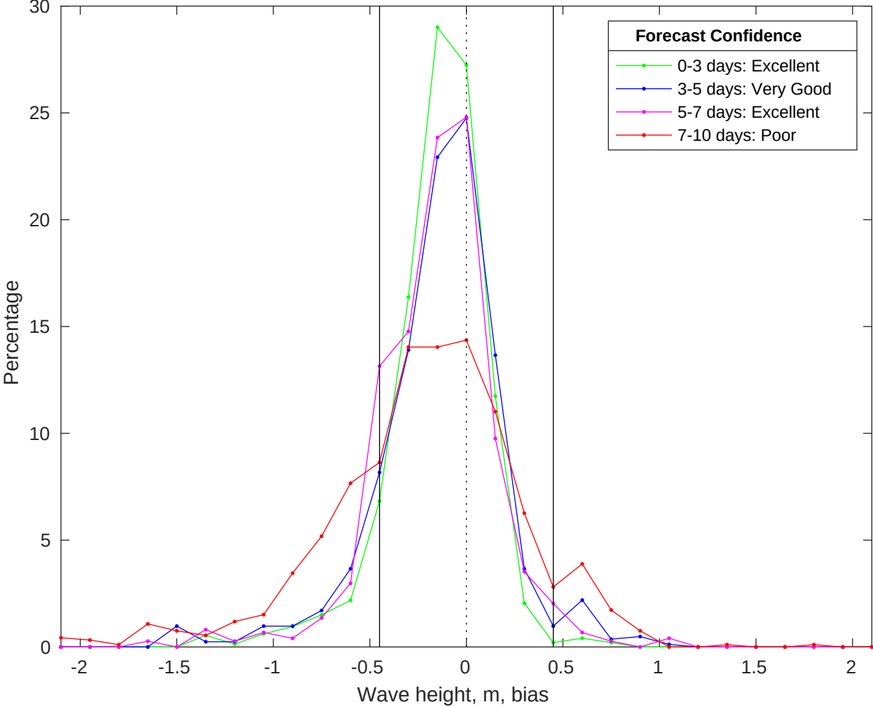
NDBC 46028 vs CMEMS Waves Bias Histogram: 06-Oct-2025
