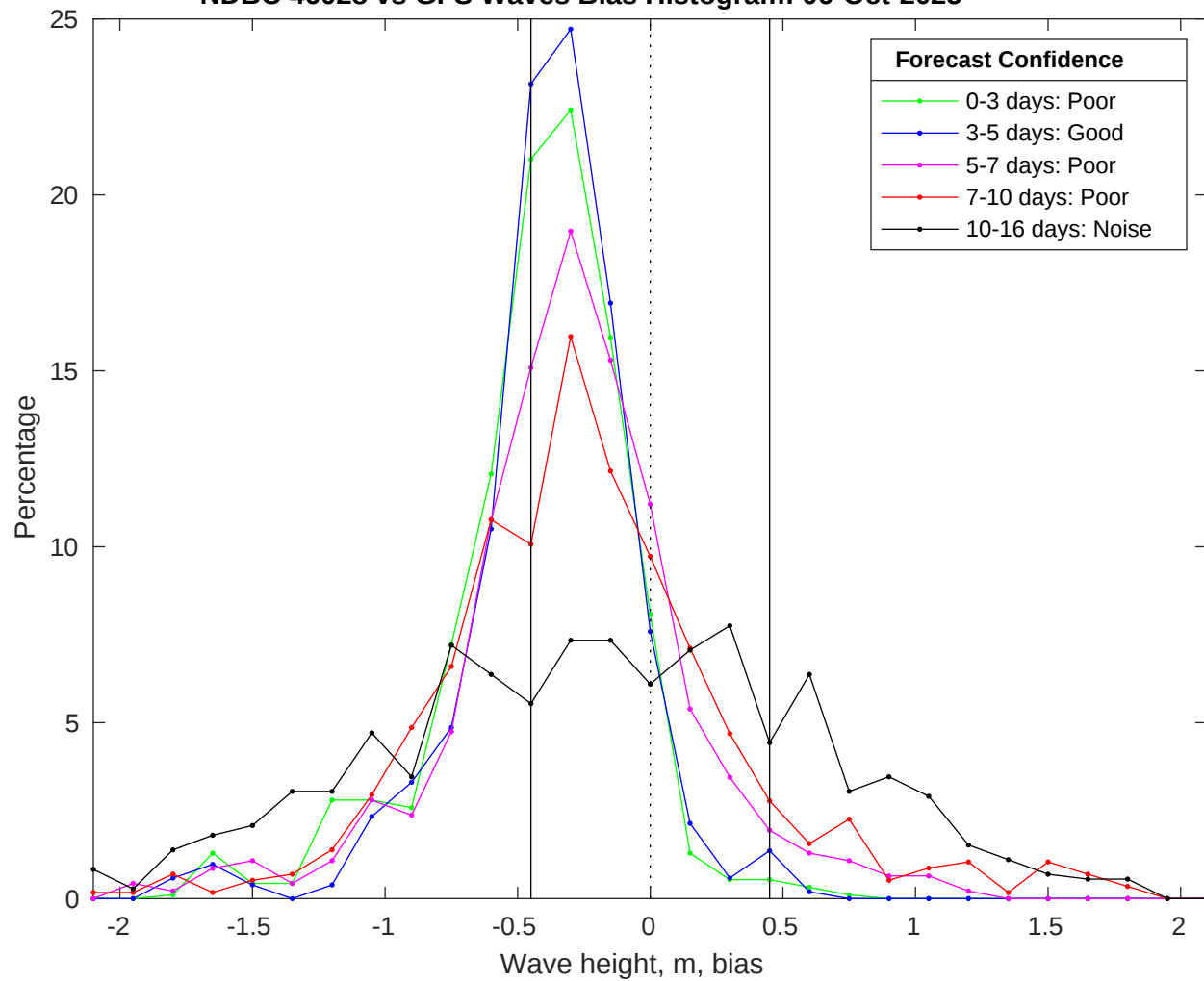
NDBC 46028 vs GFS Waves Bias Histogram: 06-Oct-2025
