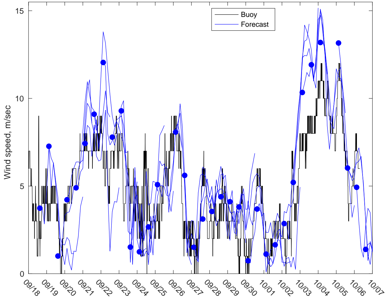
NDBC 46028 vs GFS Winds: 3 to 5 day forecast
