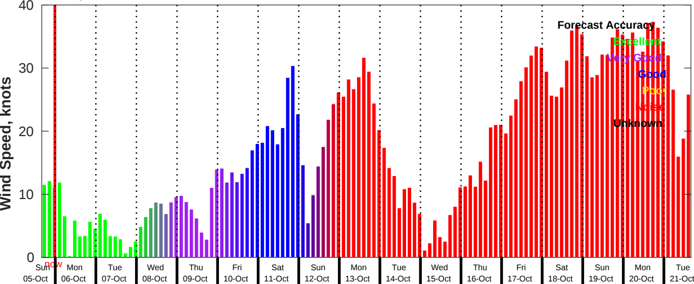
GFS Wind Speed Forecast for NDBC 46028 from 05-Oct-2025 16:00:00 to 21-Oct-2025 16:00:00
