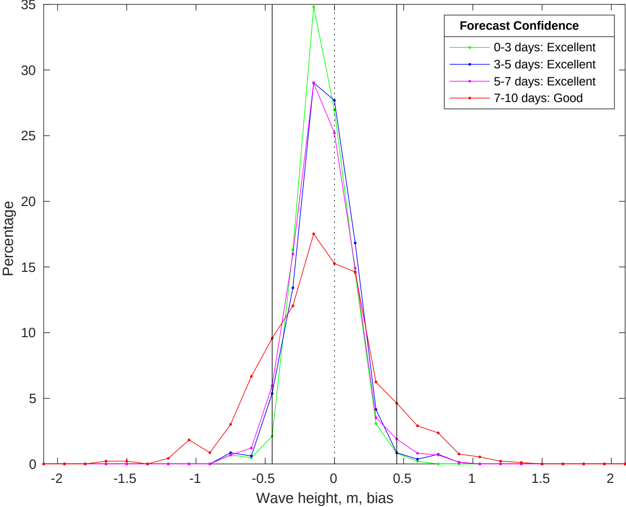
NDBC 46054 vs CMEMS Waves Bias Histogram: 06-Oct-2025
