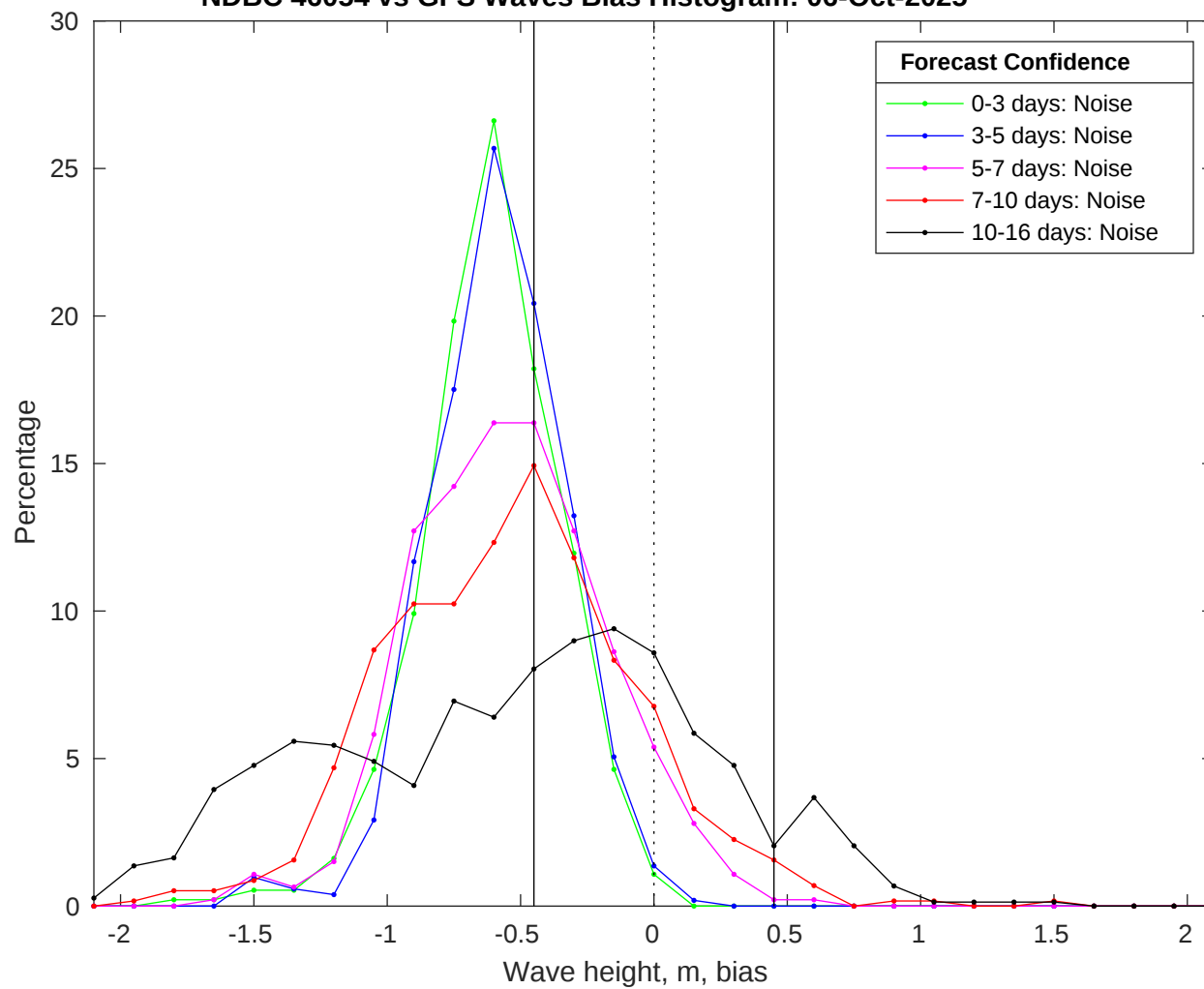
NDBC 46054 vs GFS Waves Bias Histogram: 06-Oct-2025
