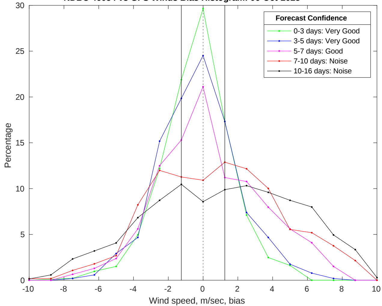
NDBC 46054 vs GFS Winds Bias Histogram: 06-Oct-2025
