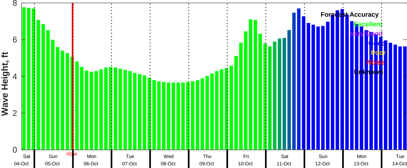
CMEMS Wave Forecast for NDBC 46054 from 04-Oct-2025 16:00:00 to 14-Oct-2025 16:00:00
