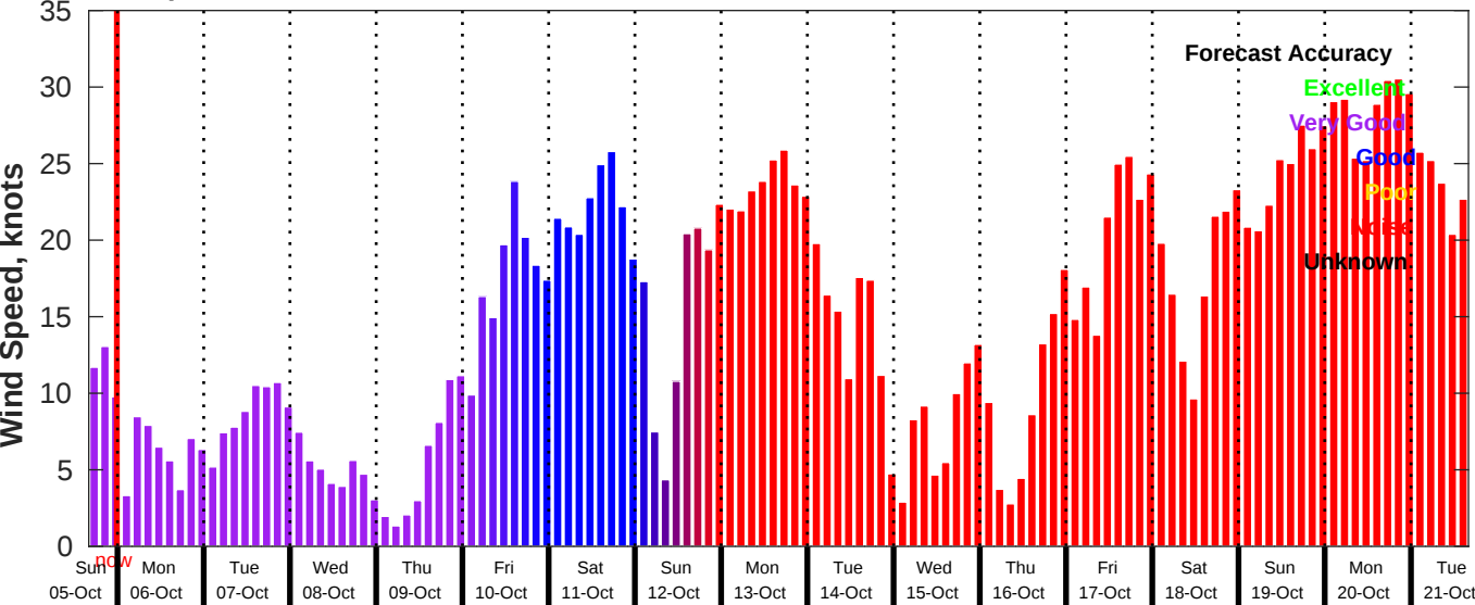
GFS Wind Speed Forecast for NDBC 46054 from 05-Oct-2025 16:00:00 to 21-Oct-2025 16:00:00
