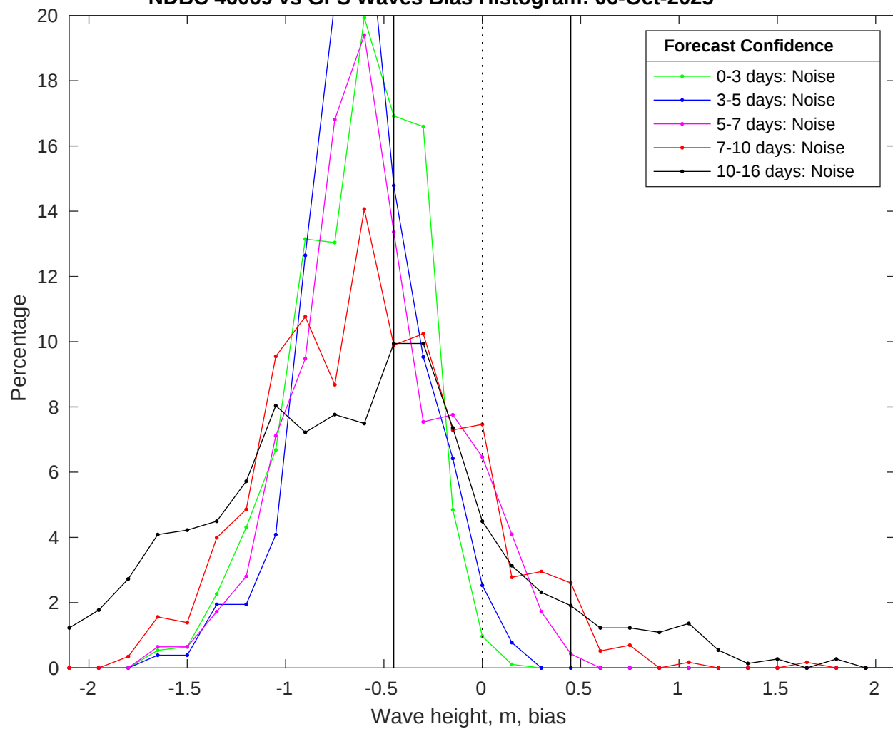
NDBC 46069 vs GFS Waves Bias Histogram: 06-Oct-2025
