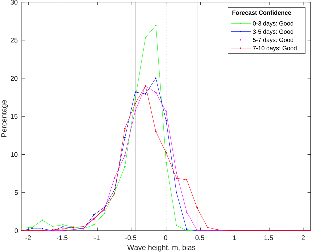
NDBC 51209 vs CMEMS Waves Bias Histogram: 06-Oct-2025
