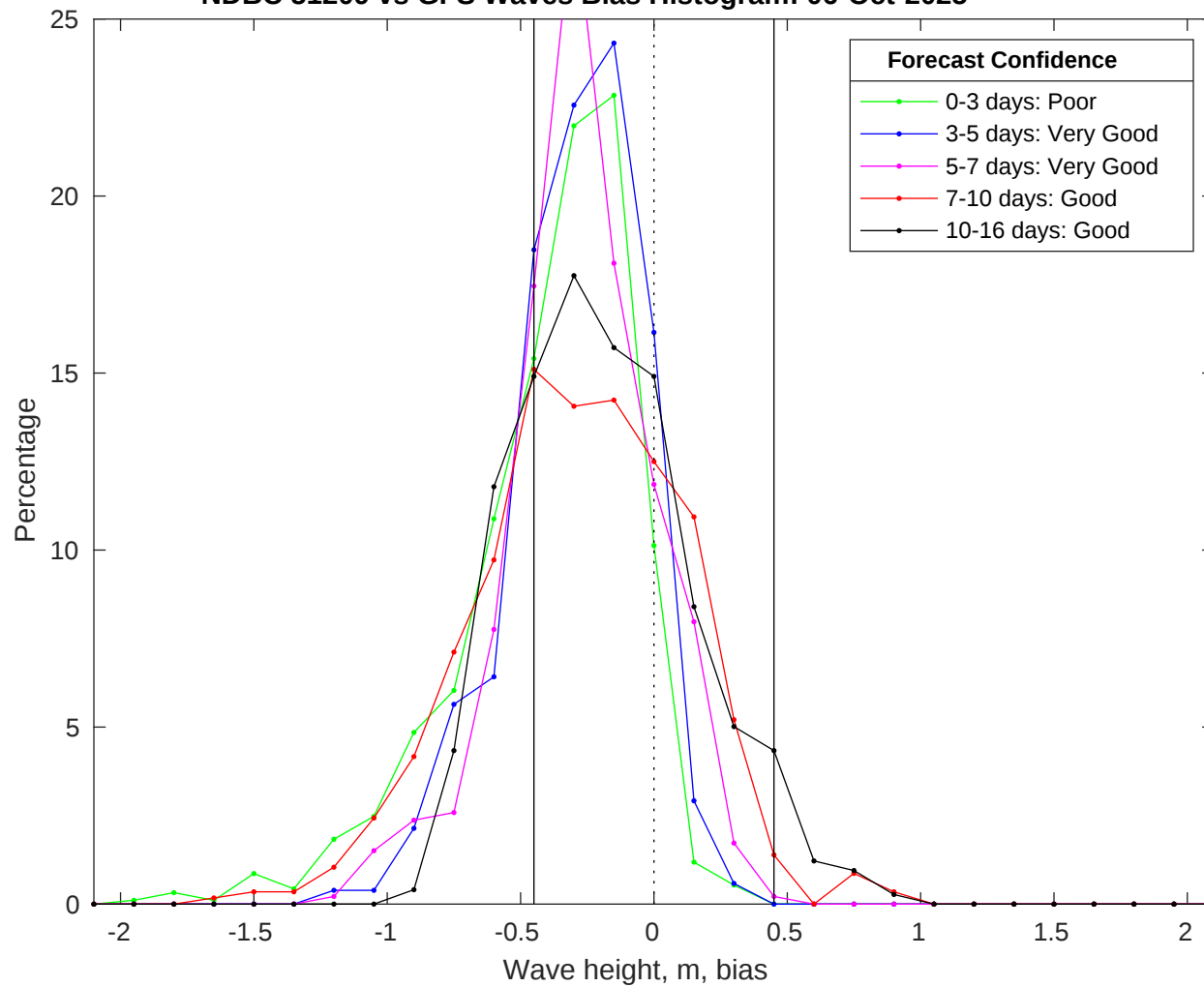
NDBC 51209 vs GFS Waves Bias Histogram: 06-Oct-2025
