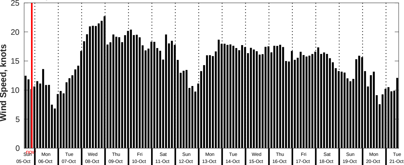
GFS Wind Speed Forecast for NDBC 51209 from 05-Oct-2025 13:00:00 to 21-Oct-2025 13:00:00
