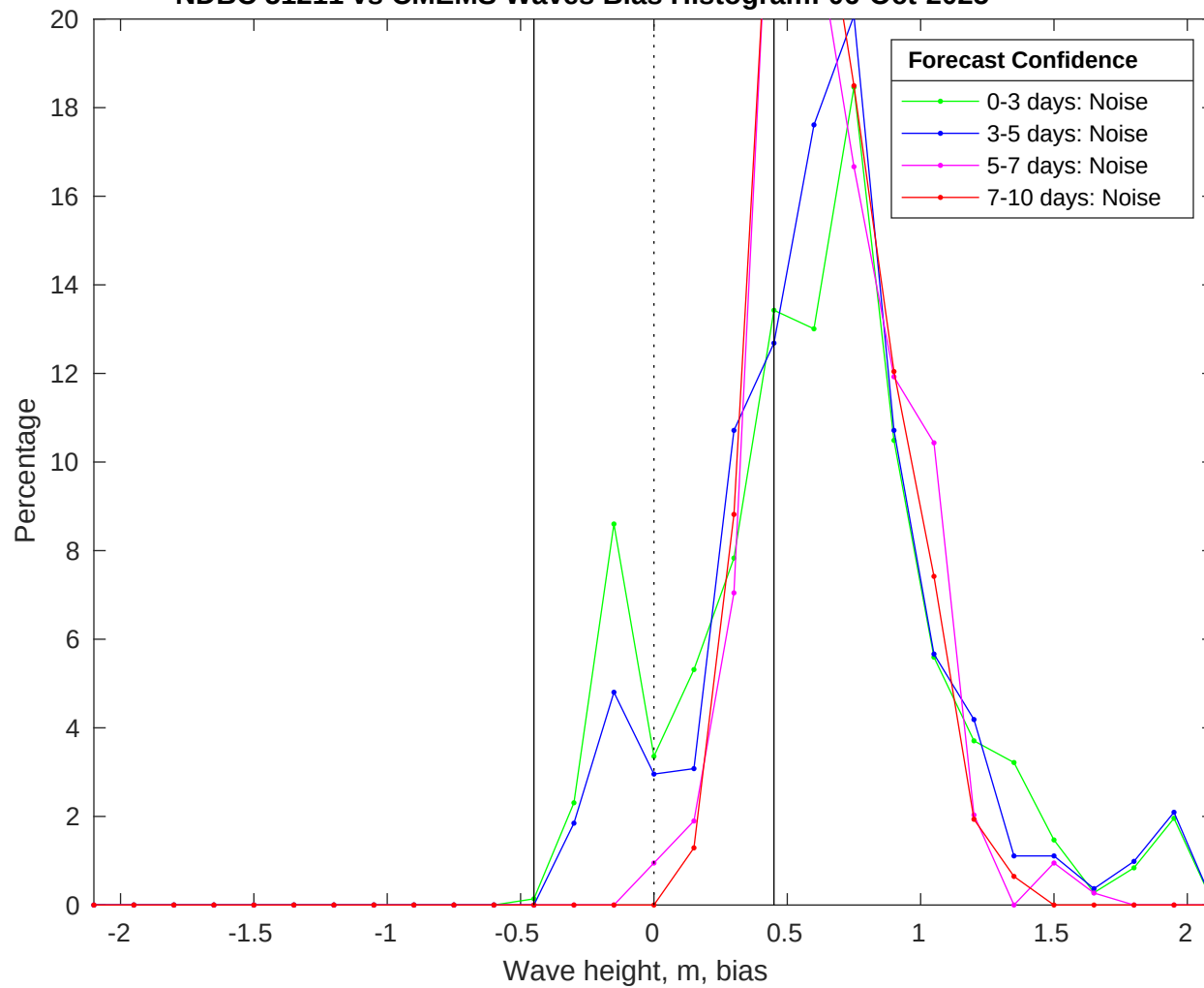
NDBC 51211 vs CMEMS Waves Bias Histogram: 06-Oct-2025
