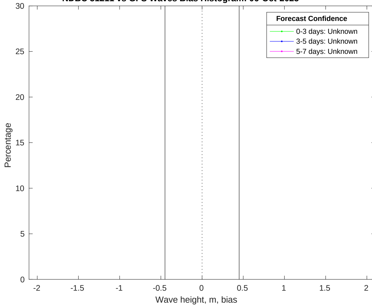
NDBC 51211 vs GFS Waves Bias Histogram: 06-Oct-2025
