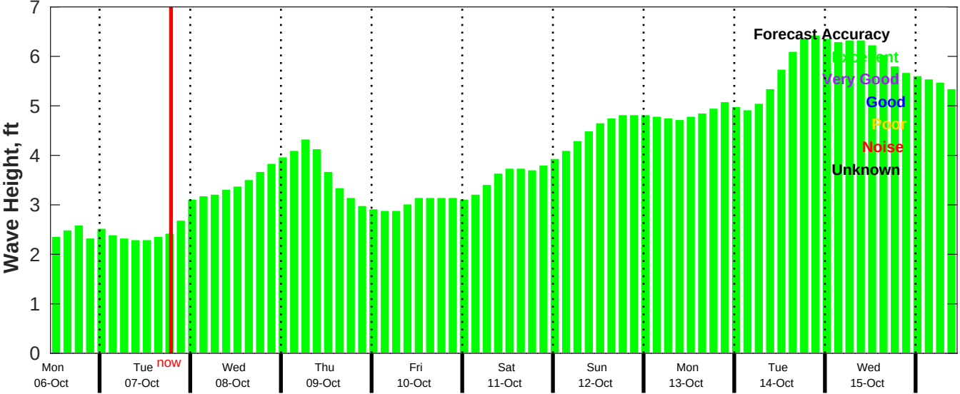
CMEMS Wave Forecast for NDBC 52211 from 05-Oct-2025 11:00:00 to 15-Oct-2025 11:00:00
