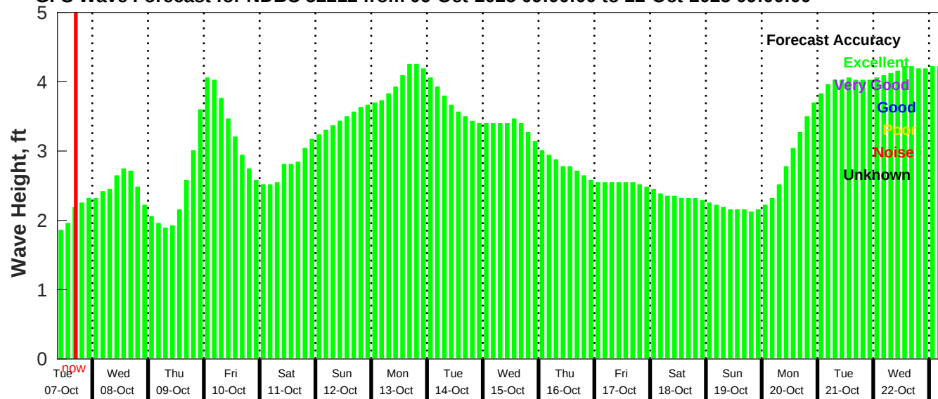
GFS Wave Forecast for NDBC 52212 from 06-Oct-2025 09:00:00 to 22-Oct-2025 09:00:00
