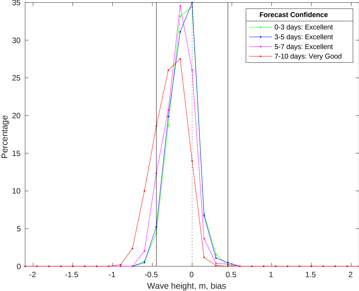
NDBC 52213 vs CMEMS Waves Bias Histogram: 06-Oct-2025
