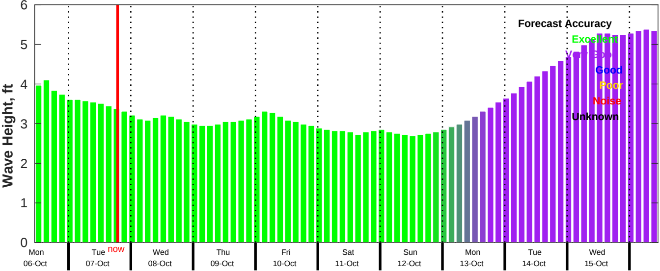
CMEMS Wave Forecast for NDBC 52213 from 05-Oct-2025 11:00:00 to 15-Oct-2025 11:00:00
