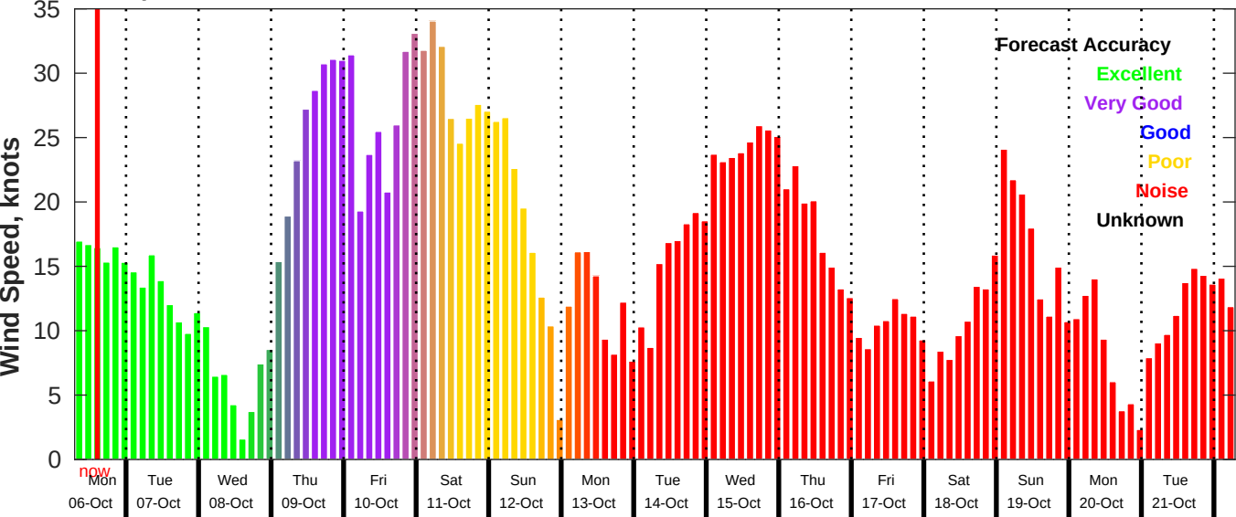
GFS Wind Speed Forecast for NDBC 41004 from 06-Oct-2025 07:00:00 to 22-Oct-2025 07:00:00
