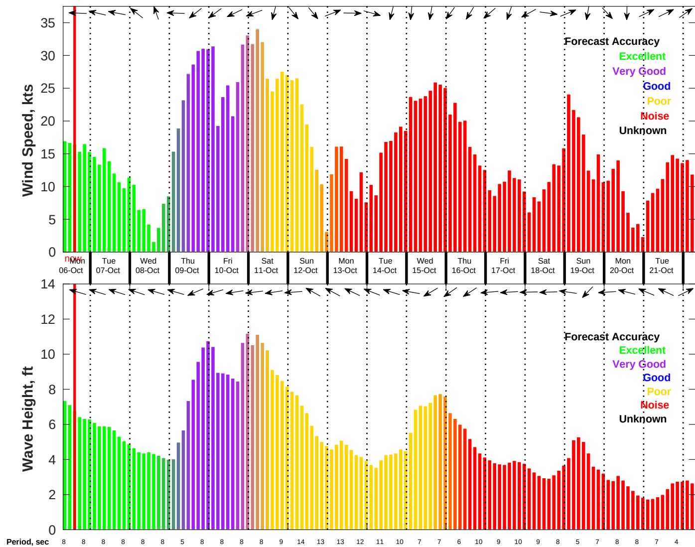
Wind & Wave Forecast for NDBC 41004 from 06-Oct-2025 07:00:00 to 22-Oct-2025 07:00:00
