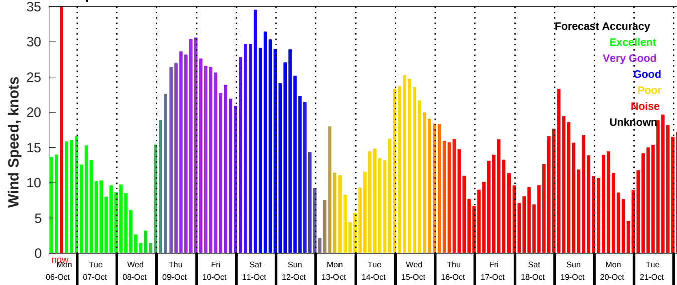
GFS Wind Speed Forecast for NDBC 41013 from 06-Oct-2025 07:00:00 to 22-Oct-2025 07:00:00
