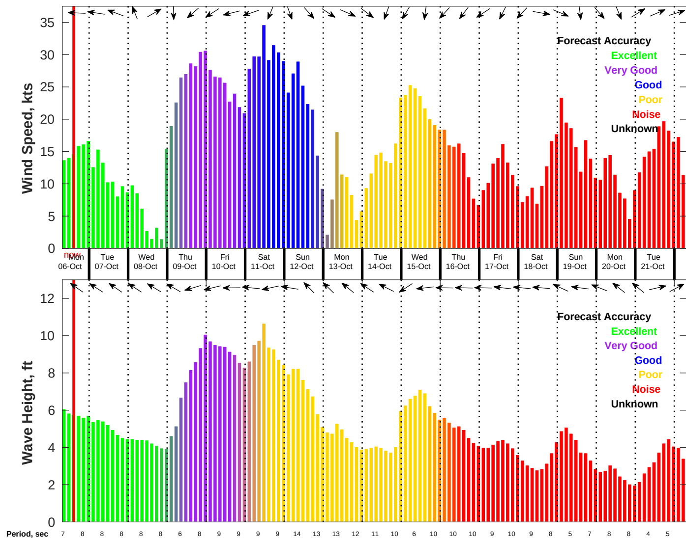
Wind & Wave Forecast for NDBC 41013 from 06-Oct-2025 07:00:00 to 22-Oct-2025 07:00:00
