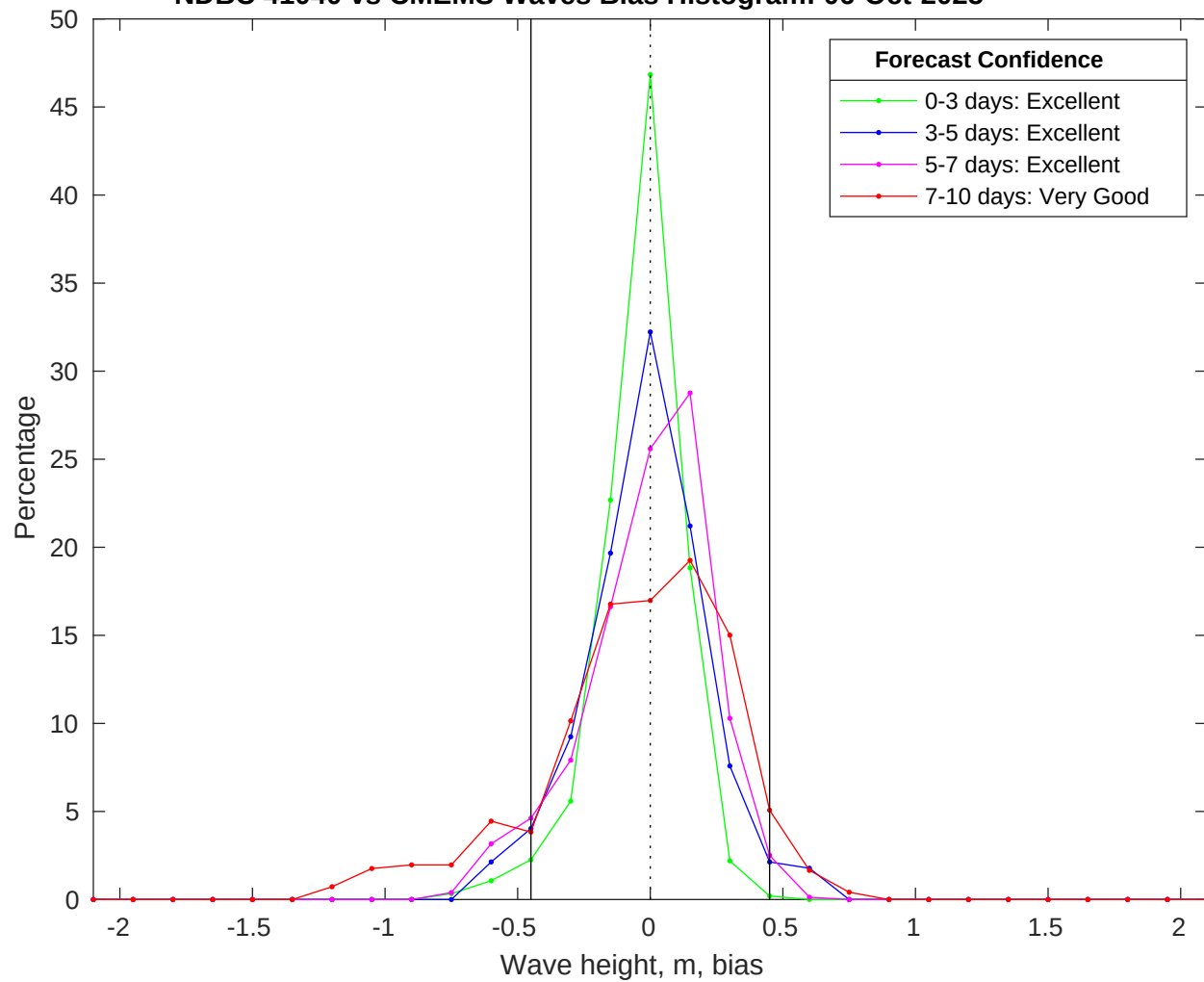
NDBC 41040 vs CMEMS Waves Bias Histogram: 06-Oct-2025
