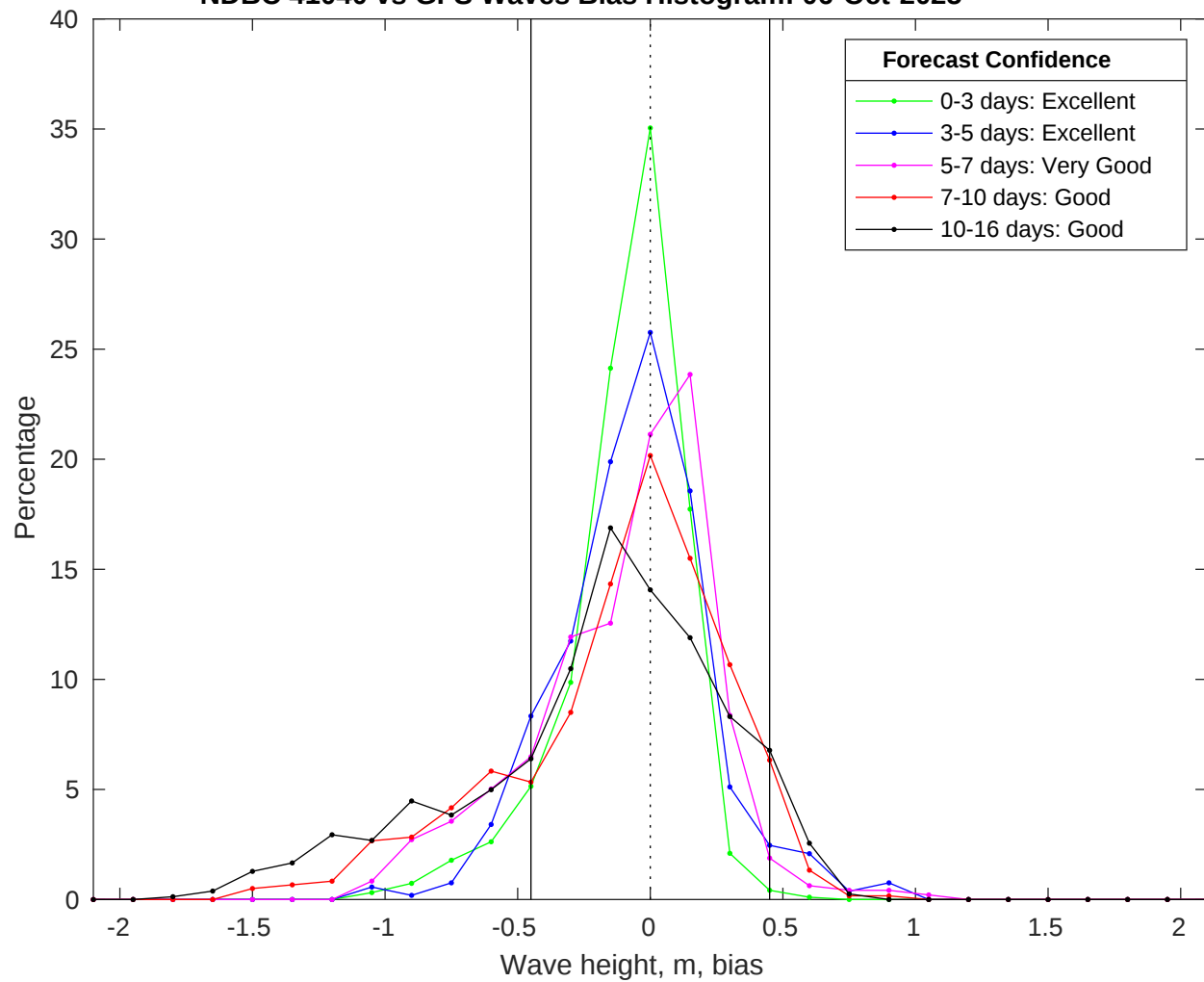
NDBC 41040 vs GFS Waves Bias Histogram: 06-Oct-2025
