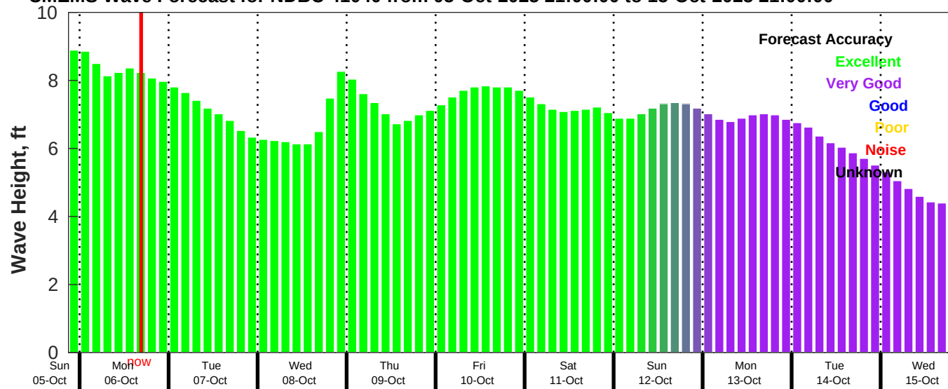
CMEMS Wave Forecast for NDBC 41040 from 05-Oct-2025 21:00:00 to 15-Oct-2025 21:00:00
