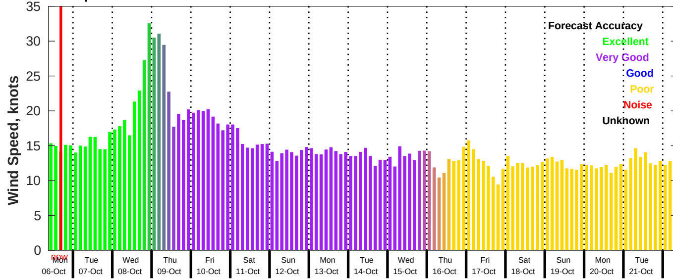
GFS Wind Speed Forecast for NDBC 41040 from 06-Oct-2025 09:00:00 to 22-Oct-2025 09:00:00
