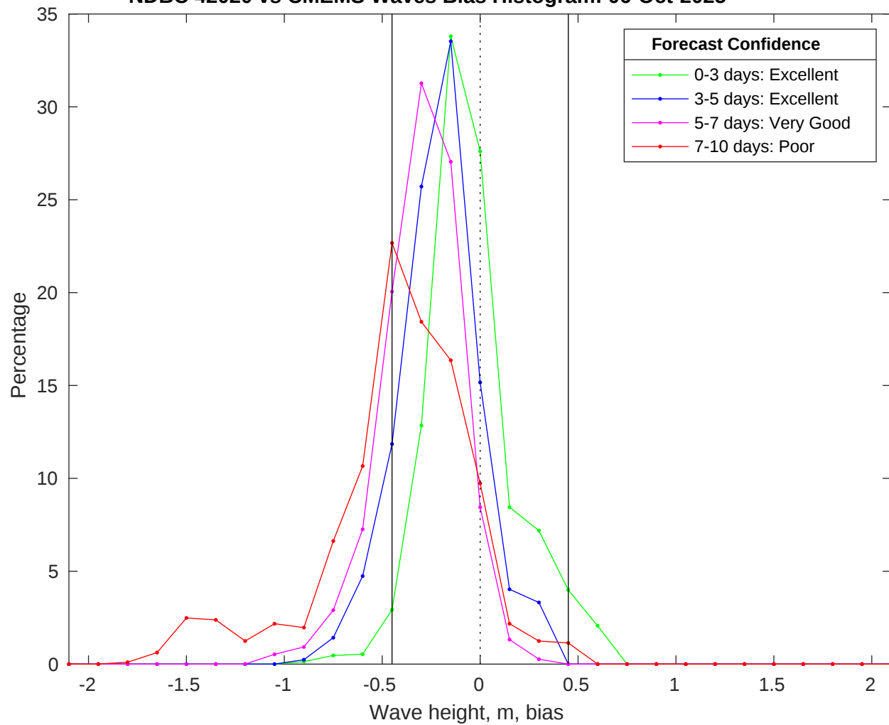
NDBC 42020 vs CMEMS Waves Bias Histogram: 06-Oct-2025
