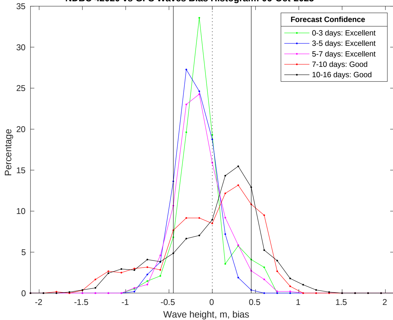
NDBC 42020 vs GFS Waves Bias Histogram: 06-Oct-2025
